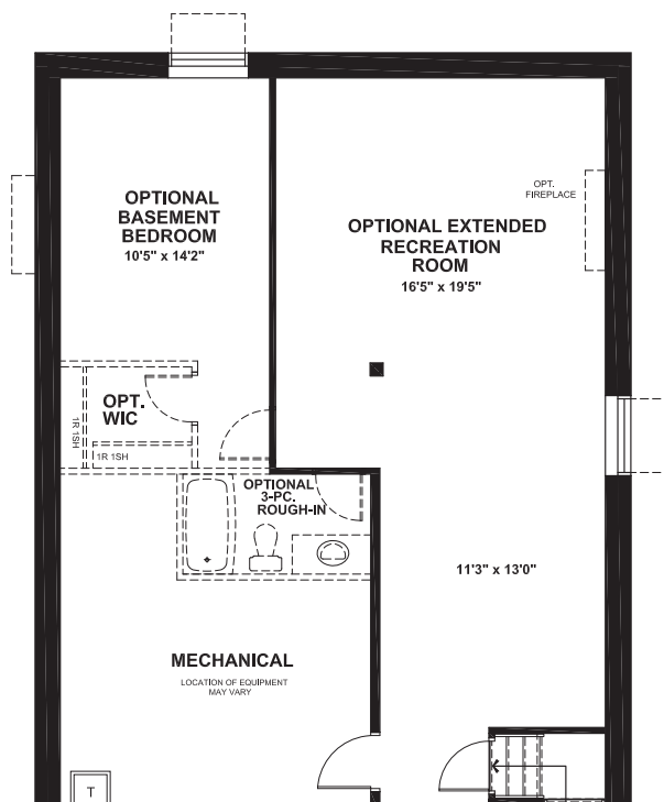
OPTIONAL BASEMENT BEDROOM AND OPTIONAL EXTENDED RECREATION ROOM
