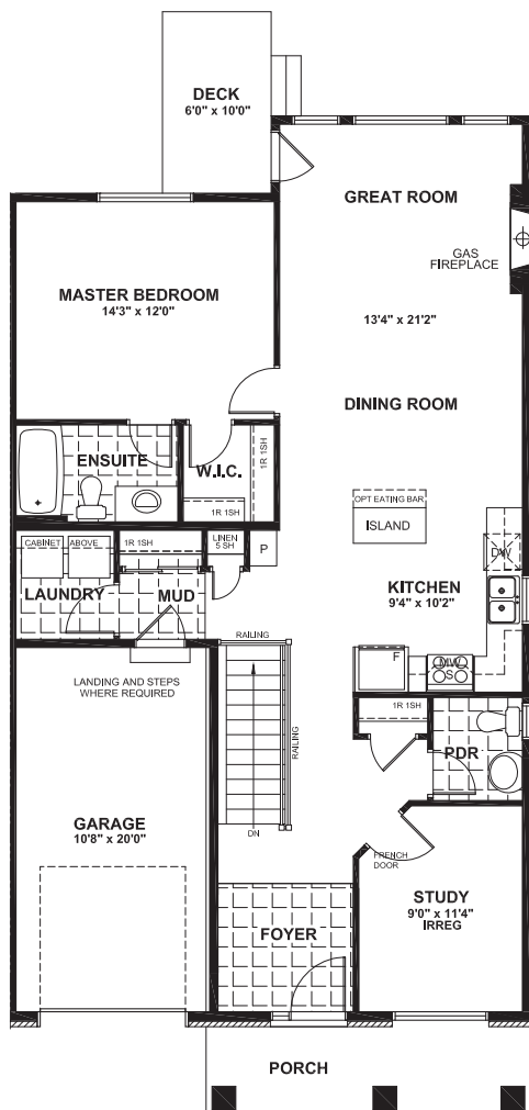
OPTIONAL GROUND FLOOR WITH STUDY – N/C
